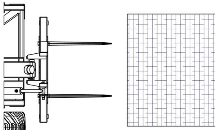
Fig.2 - Top View
